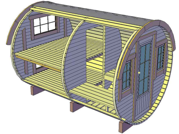
CUT VIEW
