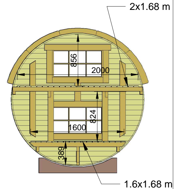
CUT VIEW
