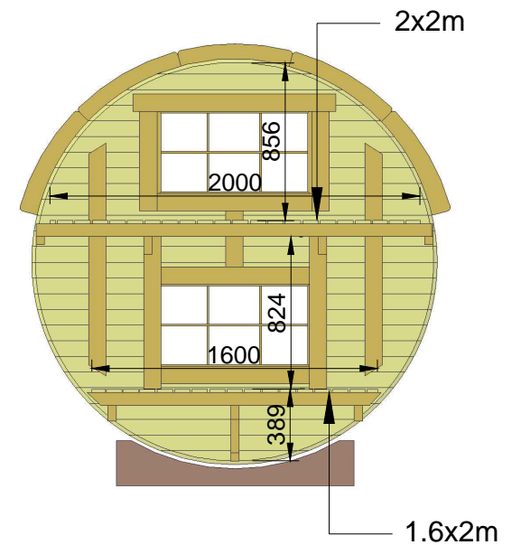
CUT VIEW
